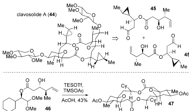
Scheme 14. Synthetic studies toward clavosolide A by Rychnovsky et al. Cy = cyclohexyl.
