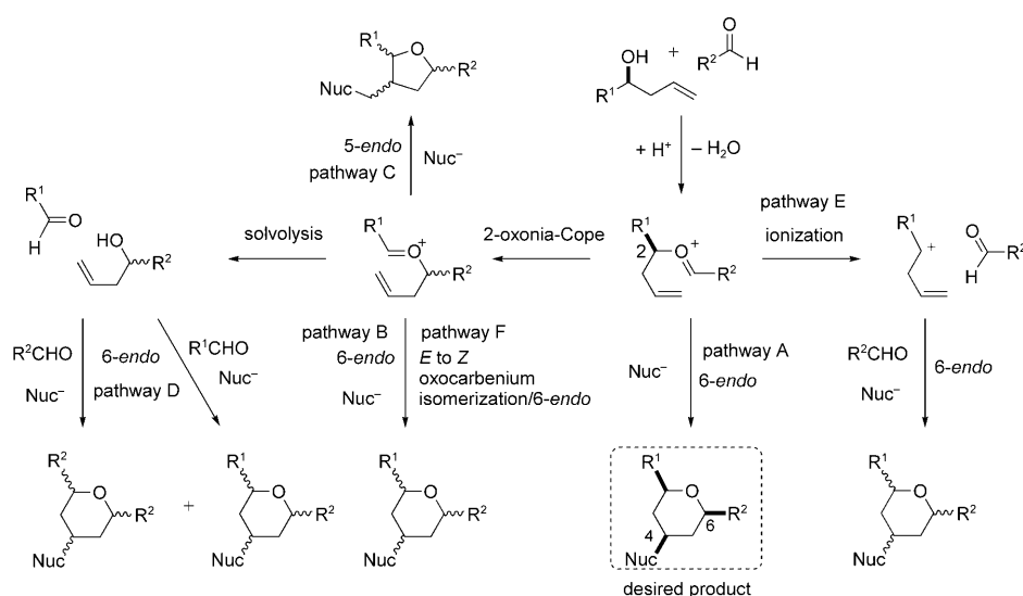
Scheme 4. Competing reaction mechanisms during Prins cyclizations to form tetrahydropyran rings.
