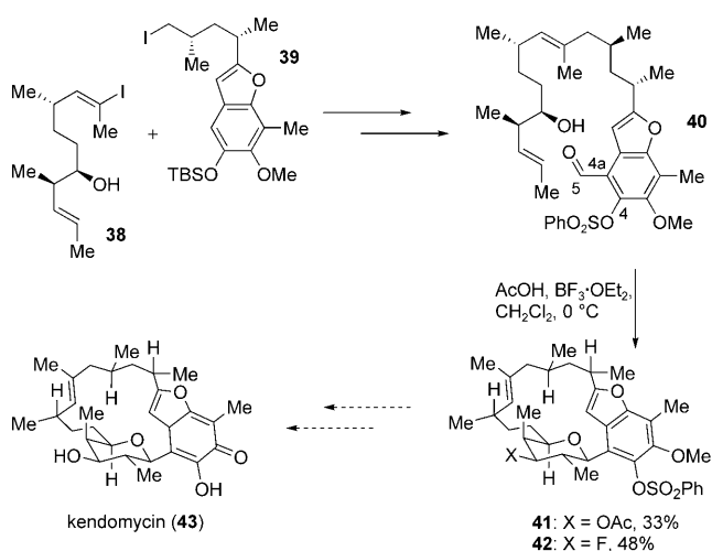
Scheme 13. Formal synthetic strategy toward kendomycin by Rychnovsky and Bahnck.
