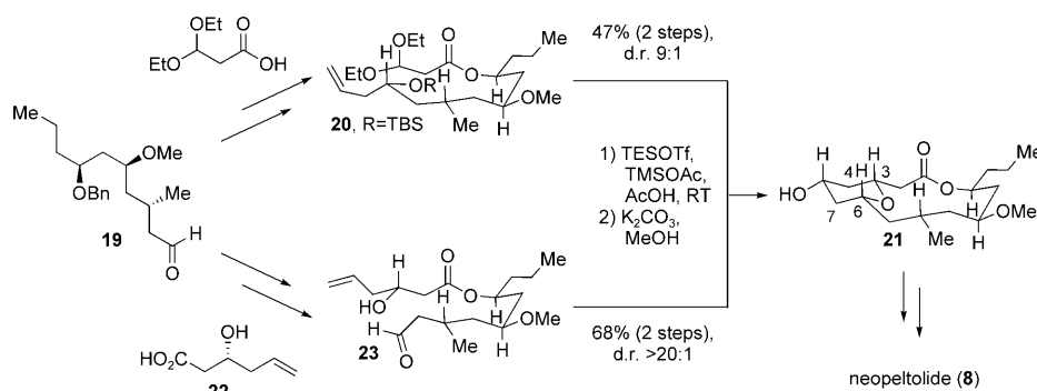
Scheme 9. Synthetic strategies toward neopeltolide by Lee et al. Bn = benzyl, TMS = trimethylsilyl.
