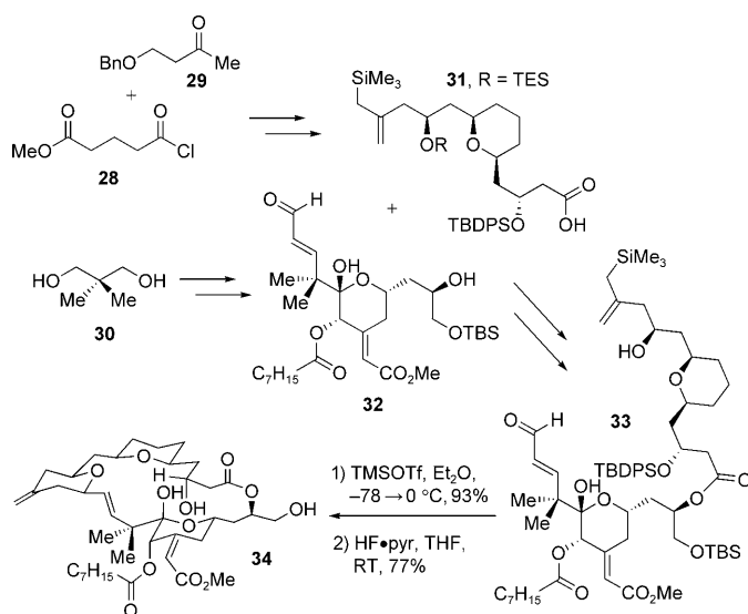
Scheme 11. Synthetic strategy toward bryostatin analogues by Wender et al. TBDPS = tert -butyldiphenylsilyl.
