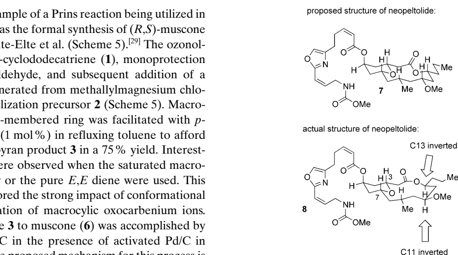
Scheme 6. The proposed and corrected structures of neopeltolide.
