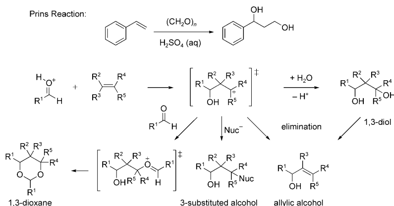
Scheme 2. The Prins reaction mechanism and possible reaction pathways. Nuc = nucleophile.
