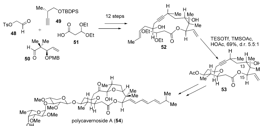
Scheme 15. Synthetic strategy toward polycavernoside A by Lee and Woo. PMB = para -methoxybenzyl.
