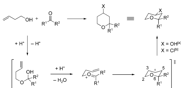
Scheme 3. The first report and mechanism of the synthesis of THP rings by the Prins reaction. [a] When \text{H}_2\text{SO}_4 was used. [b] When \text{HCl} was used.
